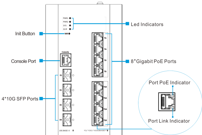
Front Panel (8-Port PoE Switch)
